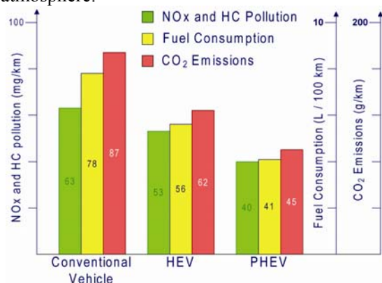
Figure 1: Vehicle Emissions and Fuel Consumption Comparison
