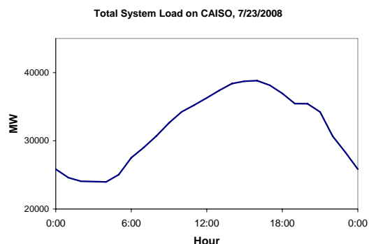
Figure 5: Summer Load Shape in California ISO on July 23, 2008 [13]
