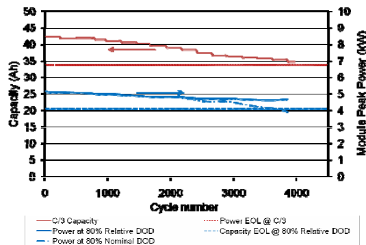
Figure 3: Deep Cycling Performance of SAFT Li Ion Battery Module Packs [5]
