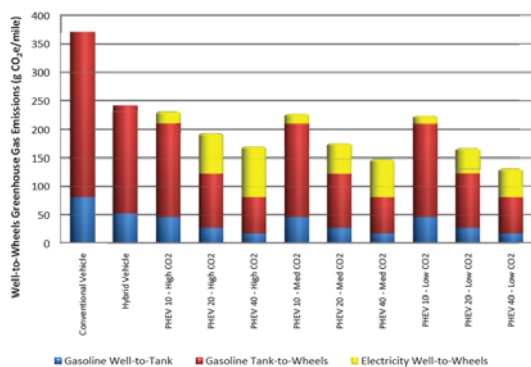
Figure 6: Greenhouse Gas Emissions for ICEVs, HEVs, and PHEVs [11]
