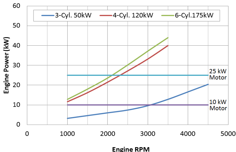
Fig.4. Minimum engine power for efficiency operation for various size engines
